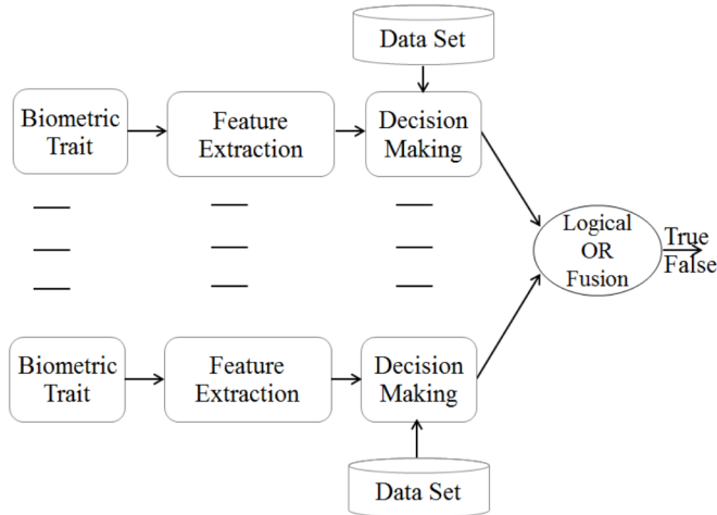
Fig. 1. Logical OR fusion method used to combine multiple biometric Traits
